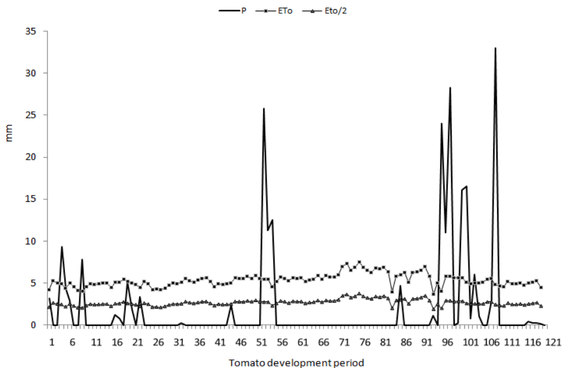
Figure 1. Rainfall, P, ETo and \frac{1}{2} ETo during the tomato development stages
